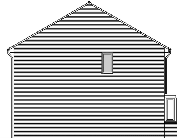
Side Elevation (Additional Side window Plot 62 Only)
